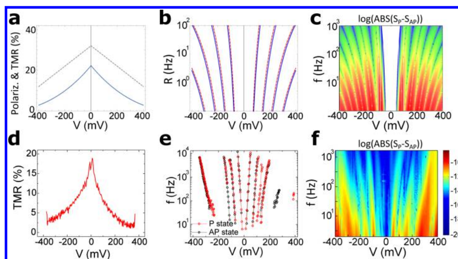
Figure 5. Comparison between LFN modeling and experiment for P and AP states. (a) Model for the electrode polarizations \mathcal{P}_\alpha(V) (dotted gray line, eq S16 in the Supporting Information) and TMR (solid blue line, eq S22 in the Supporting Information) vs applied bias. (b) Calculated switching rates R in both P (dotted red line), AP (full blue line), and unpolarized (full gray line) cases. (c) Power noise spectrum difference between P and AP states in absolute value. Measurements of (d) TMR at T = 10 K, (e) RTN characteristic frequencies in P (red dots) and AP (black dots) states at T = 10 K, and (f) power noise spectrum at T = 0.3 K. Measurements were made in the 1.2 nm thick PTCDA sample.
